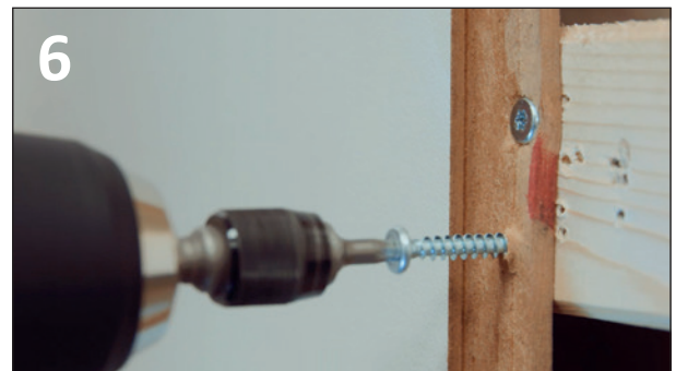
DOUBLE FIXING IN HORIZONTAL BATTENS.
