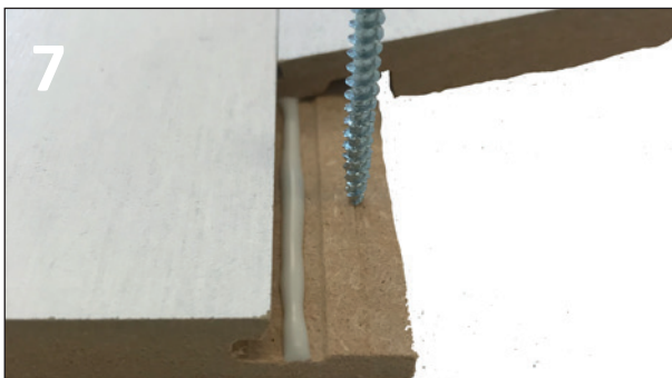
USE A 1MM STRING OF WOOD GLUE ALONG THE JOINT PROFILE. EACH PANEL MUST BE COMPLETELY FIXED TOP, BOTTOM AND SIDES BEFORE NEXT PANEL IS MOUNTED.
